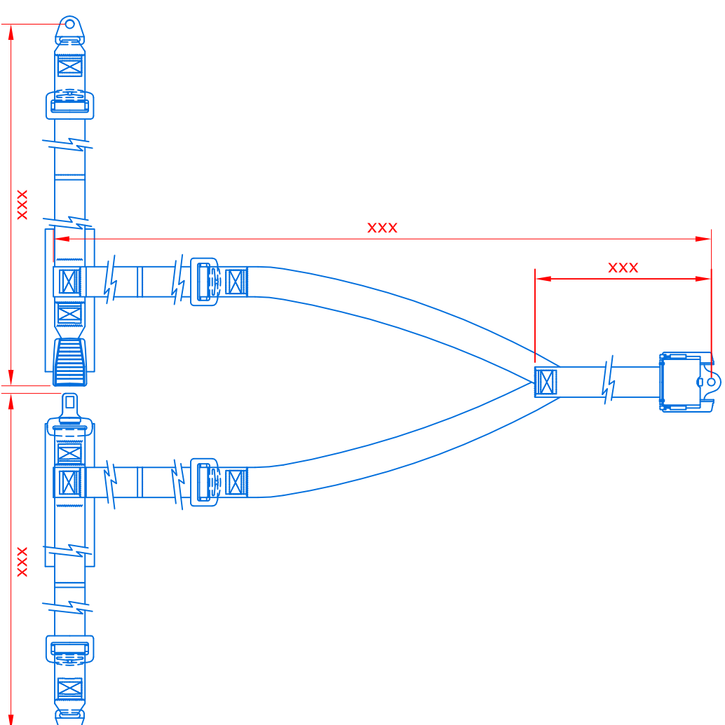
3 POINT STATIC BELT IN COMBINATION WITH THE ELR RETRACTOR
