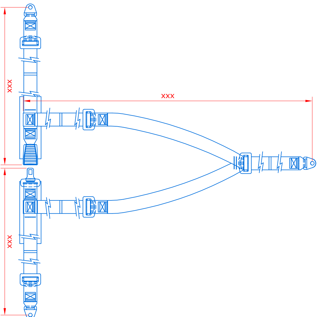
3 POINT STATIC BELT (RACING AND DISABLED PEOPLE)
